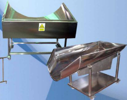
Vibrator (2modelos s/g líneas) Made of stainless steel, with wheels. It's used for drain oil of potato
