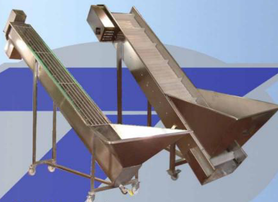
Hopper Lifting It has bearing and stainless steel frame
